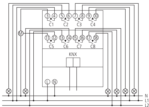
RMG 8 T KNX, RM 8 T KNX
