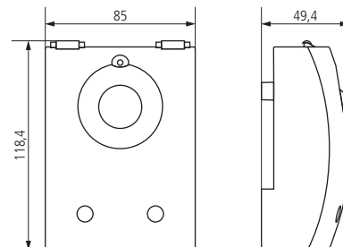
LUNA 126 star, LUNA 127 star, LUNA 128 star, LUNA 129 star-time
