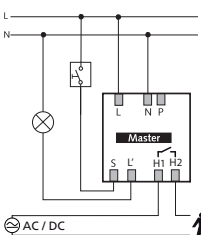
thePrema S360-101 E
