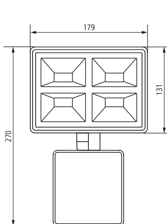
LUXA 102 FL LED 32 W
