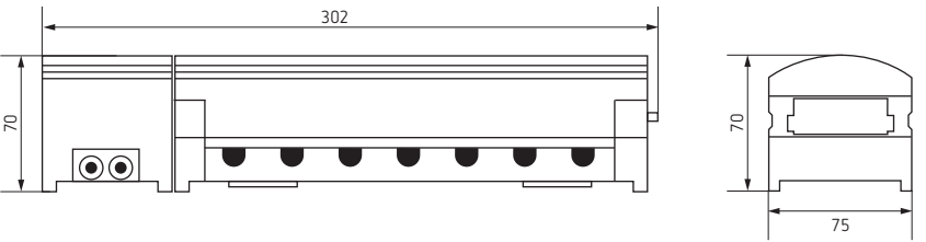
HMT 6 KNX, HMT 12 KNX
